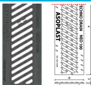
Griglia in ghisa sferoidale (fessura 10mm) Ductile iron grating (10mm slot)
