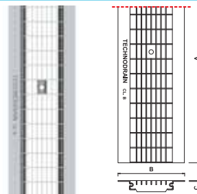
Griglia a maglia 30x10 acciaio zinc./inox Mesh 30x10 grating galvanized/s.steel
