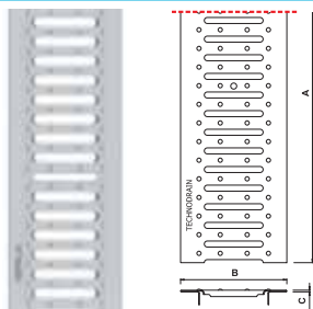
Griglia a pioli acciaio zinc./inox Slotted grating galvanized/s.steel
